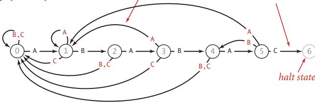
DFA corresponding to the string A B A B A C
