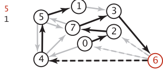
Trace of the Bellman-Ford algorithm (negative weights)
